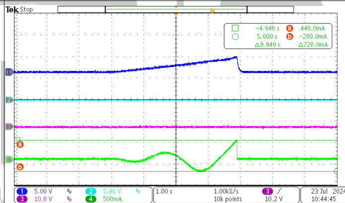
f=1000Hz, Residual Current 300mA
