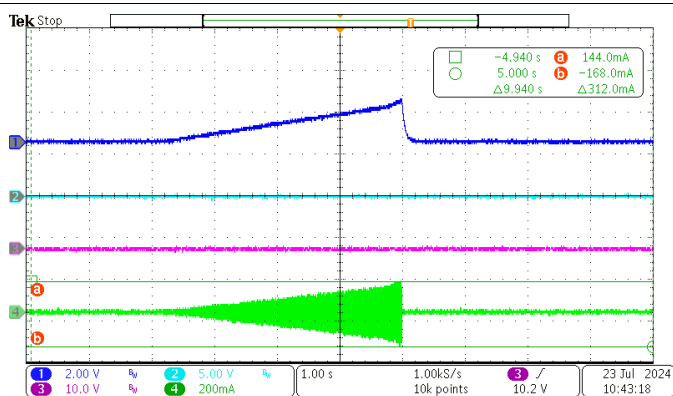
f=100Hz, Residual Current 100mA
