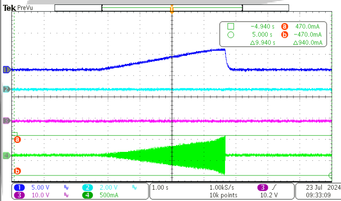
f=100Hz, Residual Current 300mA
