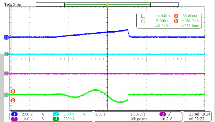
f=1000Hz, Residual Current 100mA
