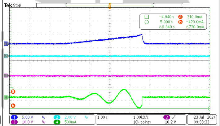
f=1000Hz, Residual Current 300mA
