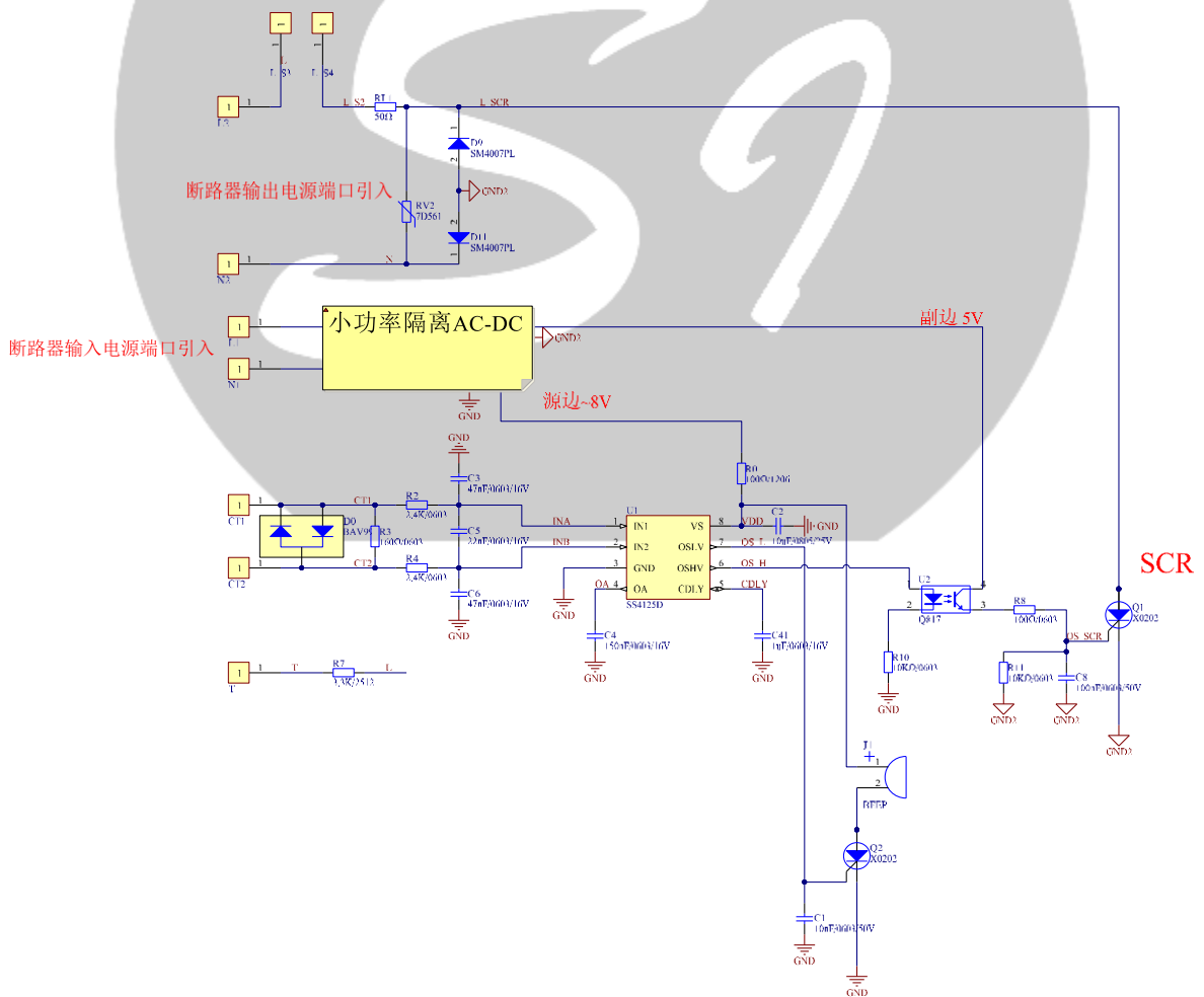
Figure 9. SS4125D high performance application with Beep Warning Rev. A | Page 7 of 17
