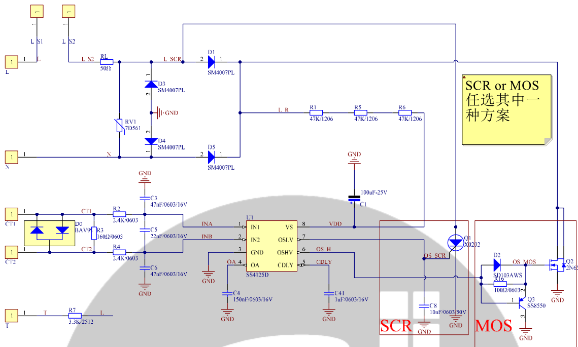
Figure 8. SS4125D high performance application
