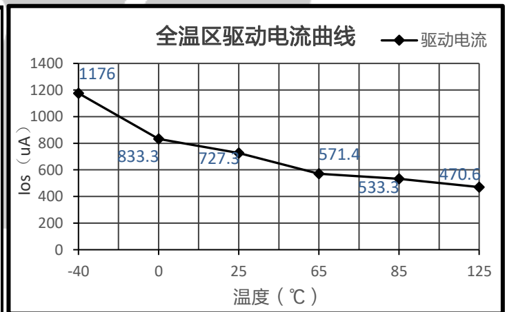
Figure3. I_{OS\_LV} Curve In -40^\circ\text{C} \sim 125^\circ\text{C}
